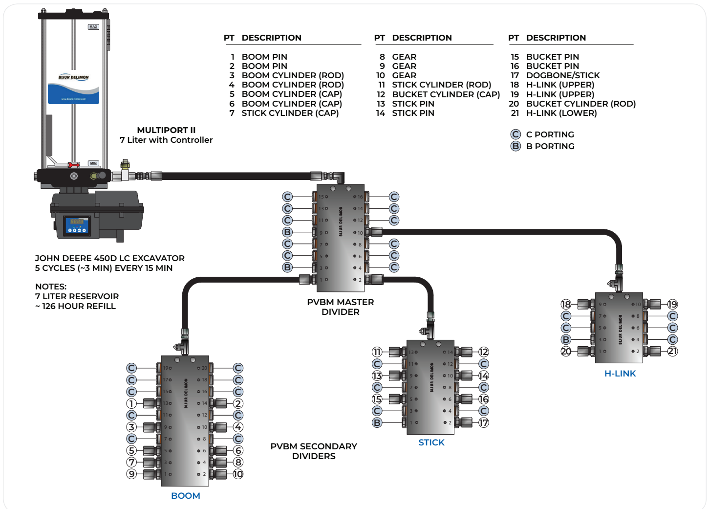
PVBM Valve
